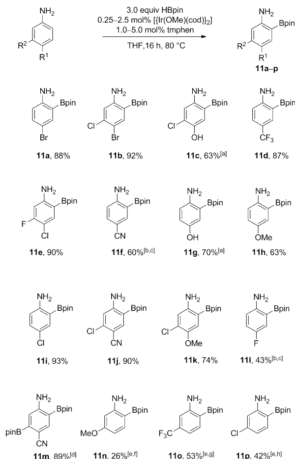
Scheme 5. Traceless Bpin-directed borylation of anilines. Yields are for isolated materials. Unless otherwise noted, the borylation catalyst was generated from Ir(OMe)(COD) 2 (0.25 mol%) and tmphen (1 mol%). See the Supporting Information for details. [a] HBpin (4 equiv). [b] HBpin (2 equiv). [c] 4,4'-bis(dimethylamino)-2,2'-dipyridyl (3 mol%) instead of tmphen; the reaction was run in hexanes with Ir(OMe)(COD) 2 (1.5 mol%). [d] The substrate is 4-aminobenzonitrile. [e] tmphen (5 mol%) and Ir(OMe)(COD) 2 (2.5 mol%). [f] Together with the 5-borylated product (47%). [g] Together with the 5-borylated product (21%). [h] Together with the 5-borylated product (17%).
